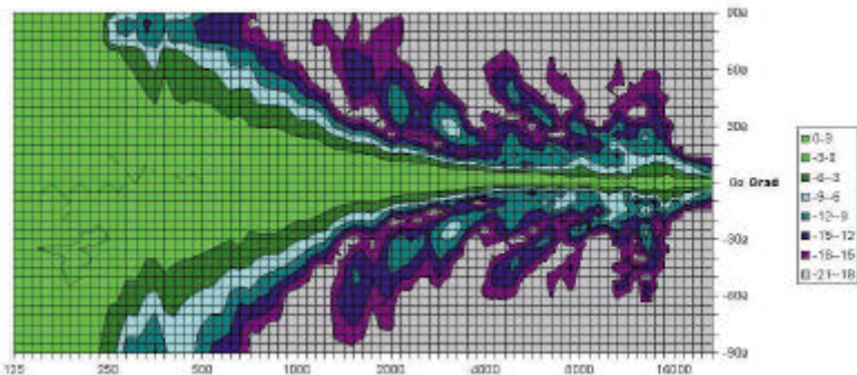
Horizontal 2D Directivity Plot SP10-Σ
