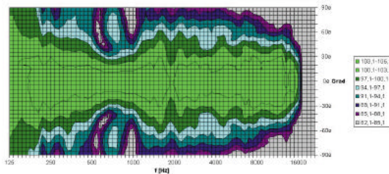
Horizontal 2D Directivity Plot SP10-Σ
