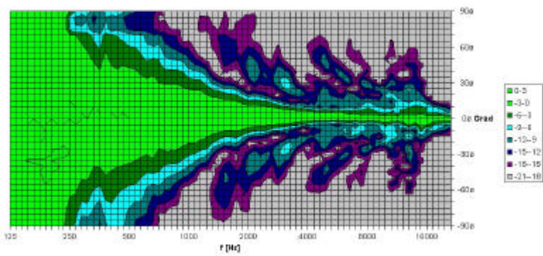
Horizontal 2D Directivity Plot SP20-Σ
