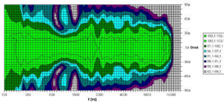
Horizontal 2D Directivity Plot SP20-Σ
