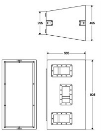
SP3-60, cabinet dimensions in mm.
