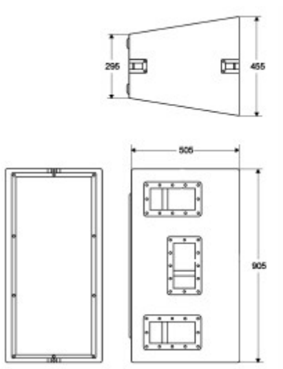
SP3-90D, cabinet dimensions in mm.
